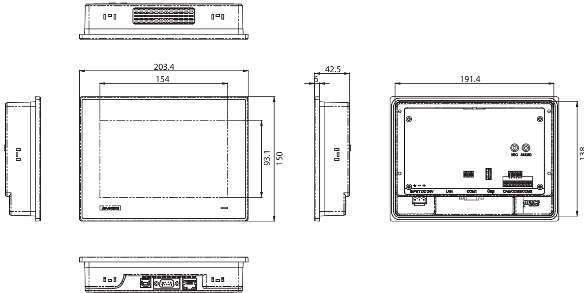
Panel Cut Out Dimensions: 192 x 138.5 mm (7.56\"/>
